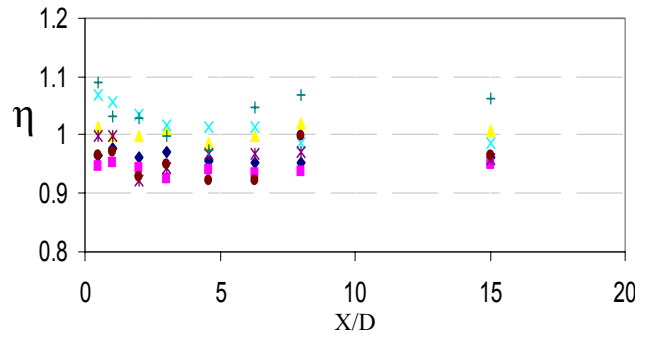
Fig. 6 Relative local Nusselt number of pulsated flow for different Re, ( f=20.7 Hz)
