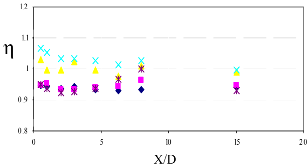
Fig. 11. Relative local Nusselt number of pulsated flow for different Re, (f=49.2 Hz)
