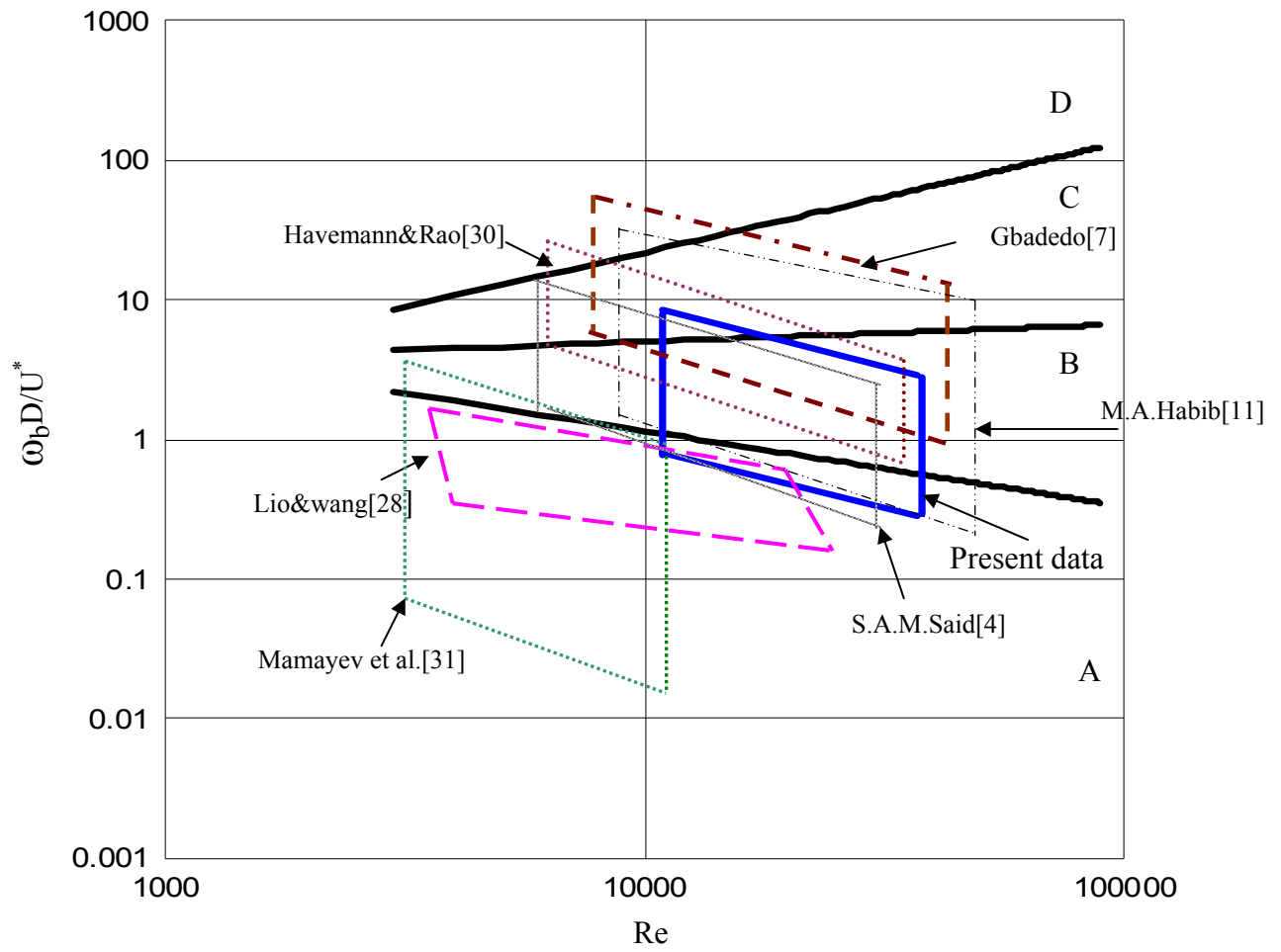
Fig.22. Classification of data of heat transfer with turbulent pulsating flow
