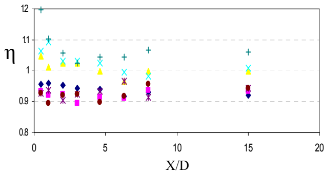
Fig. 7. Relative local Nusselt number of pulsated flow for different Re, ( f=28.3 Hz)
