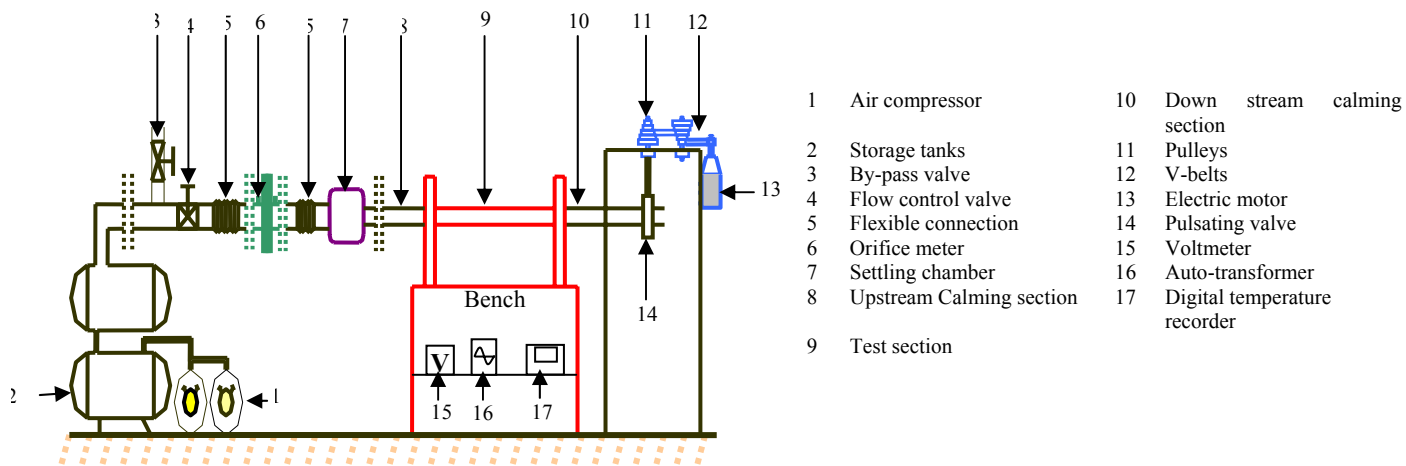
Fig. 1 Experimental equipment
