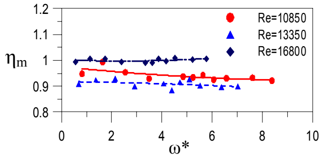
Fig .19 Relative mean Nusselt numbers as a function of dimensionless turbulent frequency.
