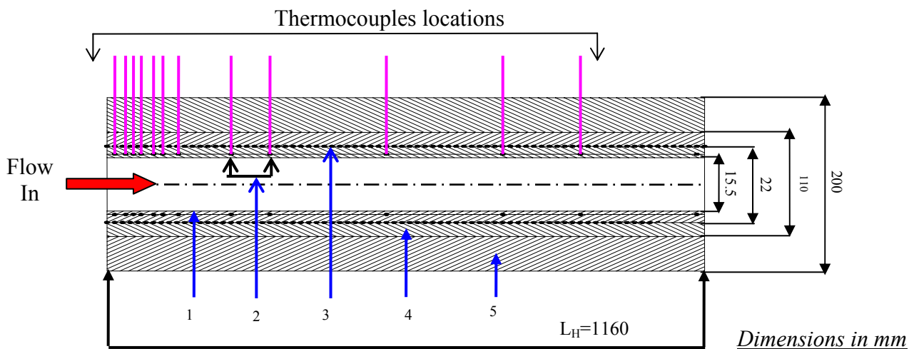
Fig. 2 Test section
