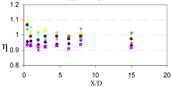
Fig. 13. Relative local Nusselt number of pulsated flow for different Re, (f=61.7 Hz)
