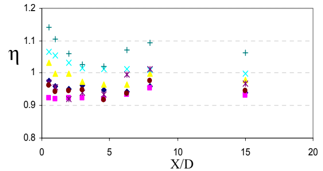
Fig. 8. Relative local Nusselt number of pulsated flow for different Re, ( f=39.3 Hz)
