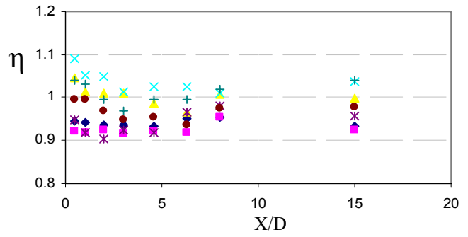
Fig. 12. Relative local Nusselt number of pulsated flow for different Re, (f=53.3 Hz)
