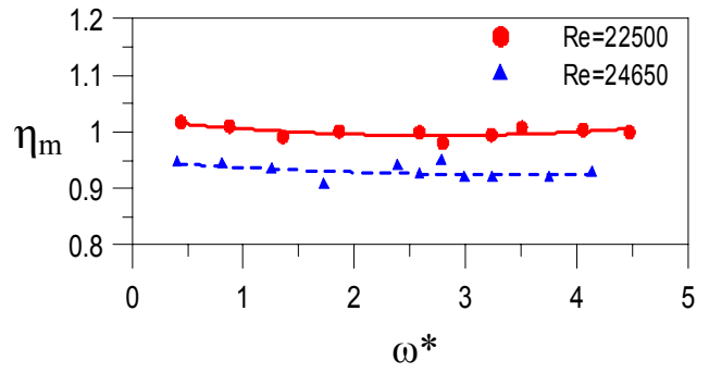
Fig .20 Relative mean Nusselt numbers as a function of dimensionless turbulent frequency.
