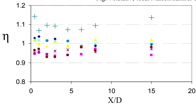
Fig. 5. Relative local Nusselt number of pulsated flow for different Re, ( f=13.3 Hz)
