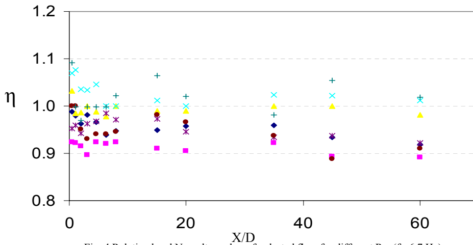
Fig. 4 Relative local Nusselt number of pulsated flow for different Re, ( f=6.7 Hz)
