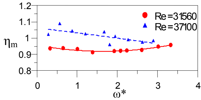
Fig .21 Relative mean Nusselt numbers as a function of dimensionless turbulent frequency.
