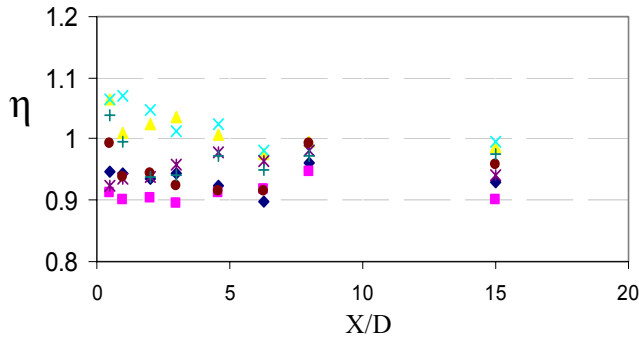
Fig. 9 Relative local Nusselt number of pulsated flow for different Re, ( f=42.5 Hz)
