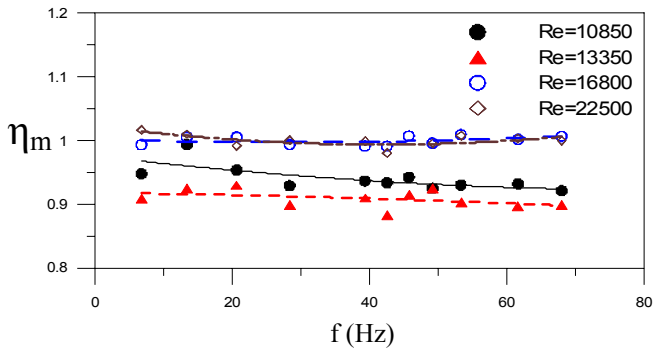
Fig. 15. Relative mean Nusselt number as a function of pulsation frequency.
