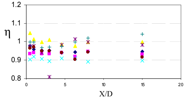
Fig. 10 Relative local Nusselt number of pulsated flow for different Re, ( f=45.7 Hz)
