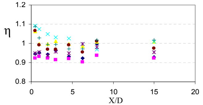
Fig. 14. Relative local Nusselt number of pulsated flow for different Re, (f=68 Hz)
